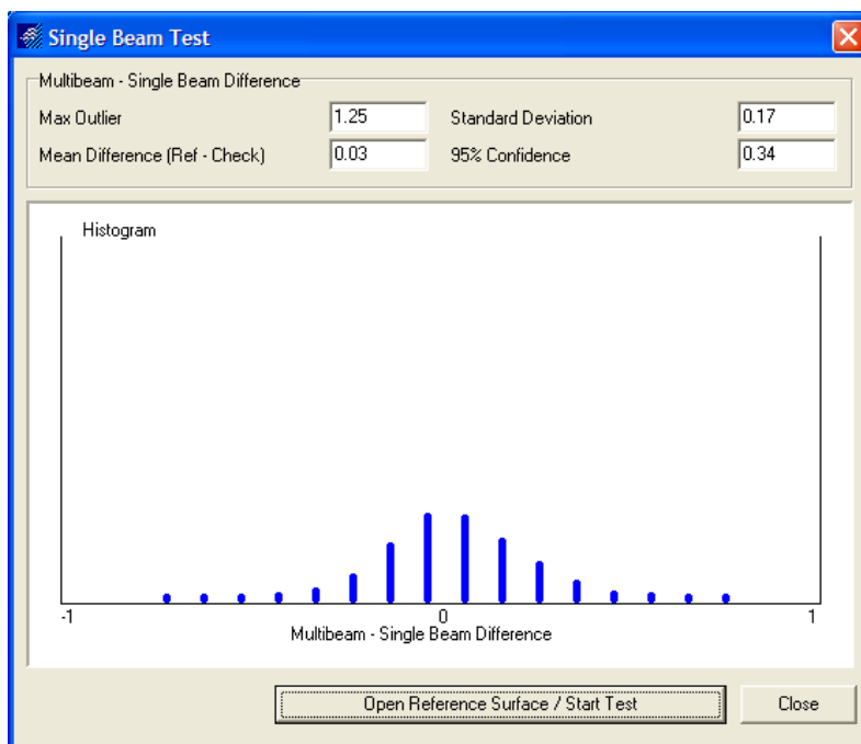
Figure F-6. Shuman Multibeam vs. S/V Cherneski Single Beam: Single beam 0.03' shallower.
