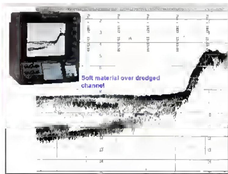
Figure P-11. Teledyne Odom Hydrographic ECHOTRAC MKIII dual frequency thermal echo sounder (24 kHz and 200 kHz), depicting soft sediment material over dredged channel.
